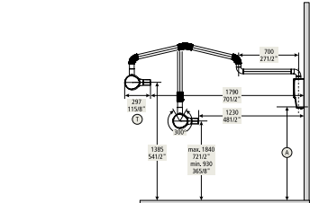
Heliodent Plus, long support arm*
