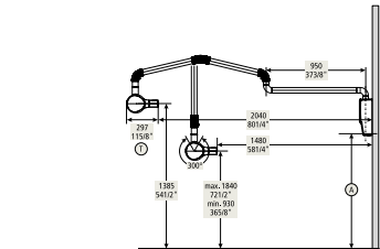
Heliodent Plus, extra long support arm*
